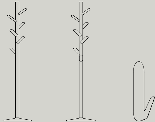
Coat Stand with 6 hooks W 412 H 1700 D 412 Coat Stand with 8 hooks W 412 H 1700 D 412 Coat Hook W 55 H 412 D 55
