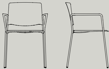
4 Legs armchair W560 H810 D589
